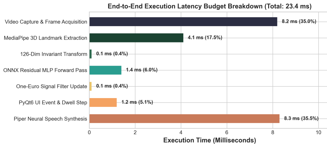
Figure 6.2: End-to-End System Execution Latency Budget Breakdown: Measured latency across each pipeline stage, totaling just 23.4 ms (well below the 50 ms interactive ceiling).
